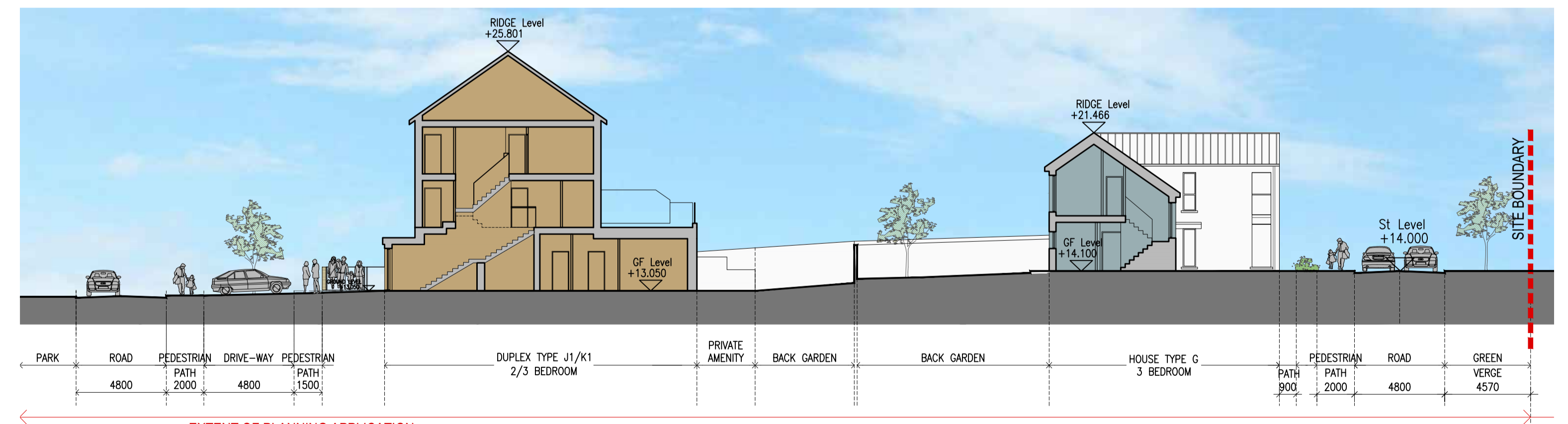
SECTION D
