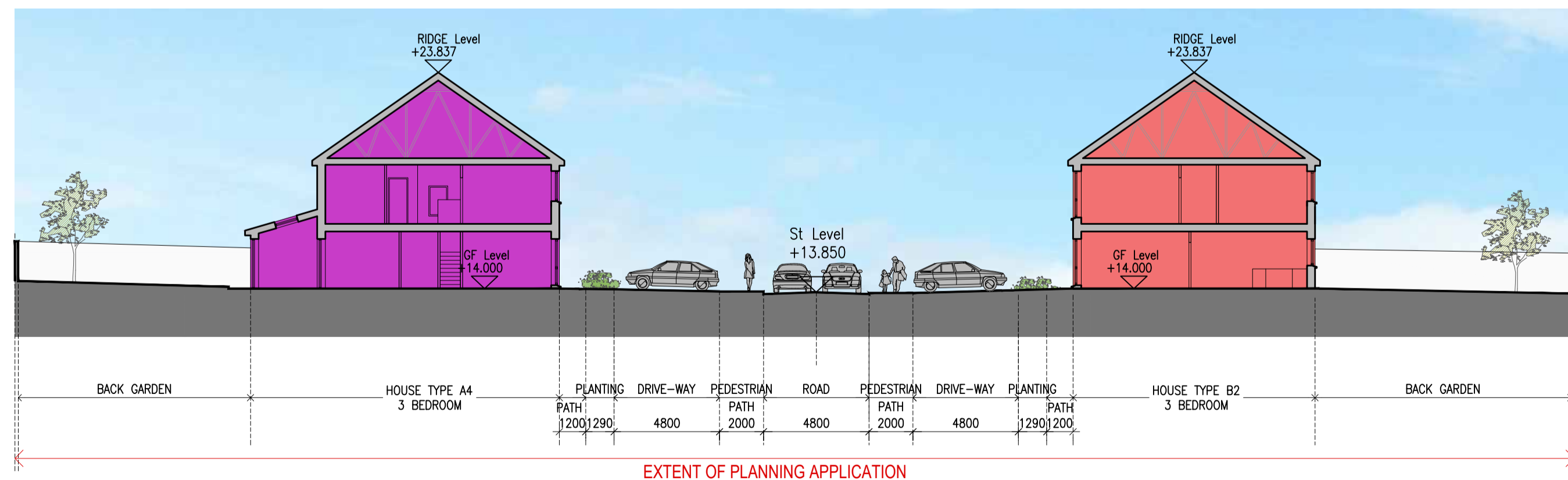
SECTION C
